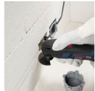
Routing grooves in porous concrete, for laying concealed cables and pipes.
