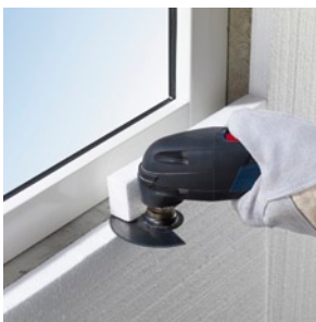
Flush cutting to length of protruding insulation material, e.g. polystyrene.
