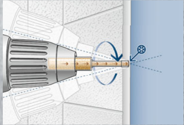
Drill through the tile using slight circular motion.
