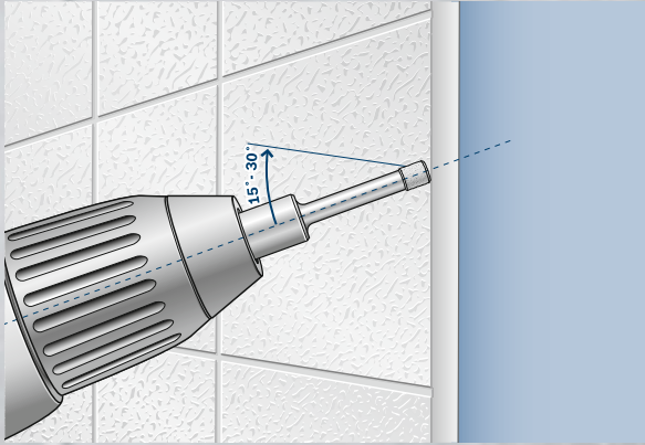
Apply the drill bit at an incline to start drilling (angle of 15° to 30°) and gradually straighten it up.
