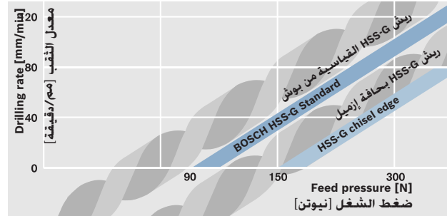
Metal drill bits HSS-G: up to 40% faster or 50% less feed pressure
